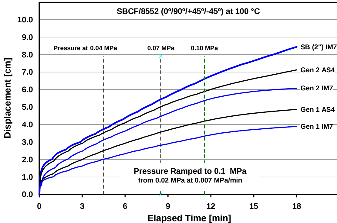
Figure 10: Bulge Test Displacement Curves of Gen 1 and 2 SB AS4/8552 preregs and SB (2.0'') IM7/8552 prepreg
