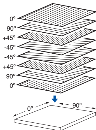
■ Quasi-isotropic lay-up
