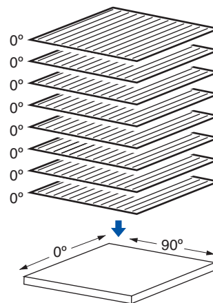
■ Unidirectional lay-up
