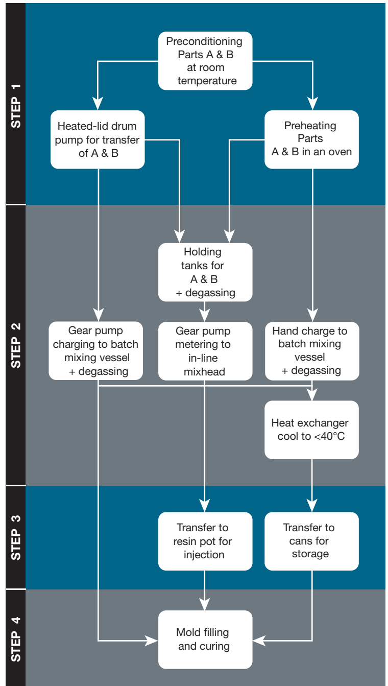
Figure 1–Typical RTM200 resin processing steps
