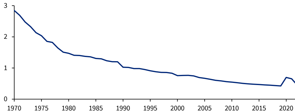
Aviation industry fuel efficiency 1, 2 Pounds of CO 2 per revenue-passenger-mile
