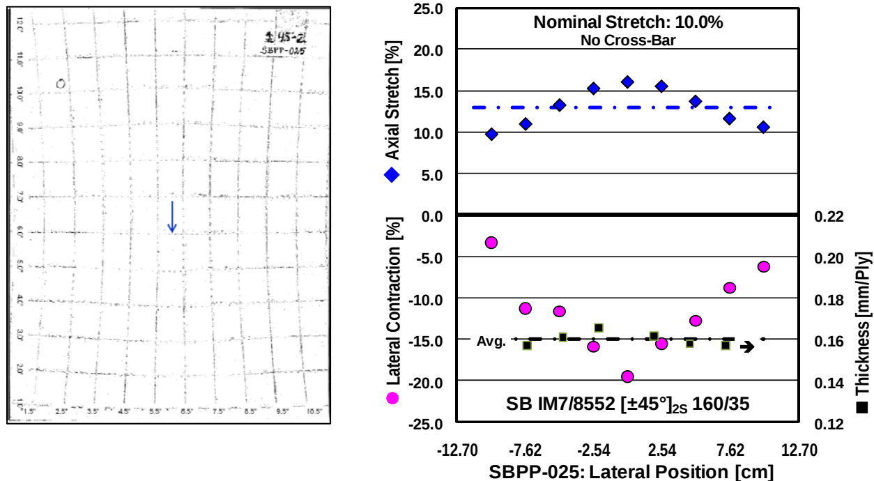
Figure 6: \pm 45^\circ Panel SBPP-025 Stretched at Prepreg Level by Overall 10% Grid Lines (Left) and Evaluation Results (Right)
