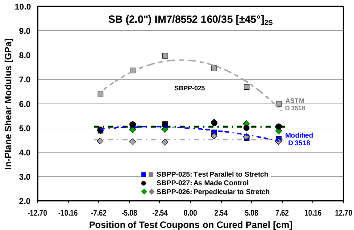
Figure 9. In-Plane Shear Modulus of 8-Ply \pm 45 Panels SBPP-025 to -027
