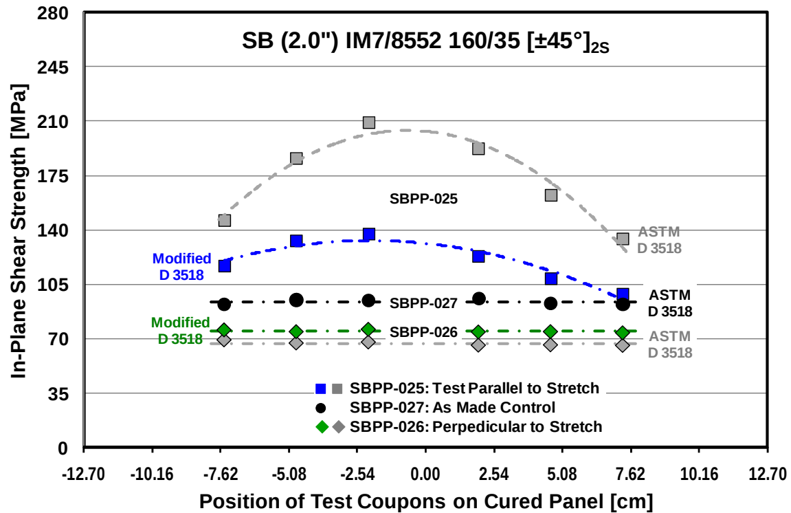
Figure 8: In-Plane Shear Strength of 8-Ply \pm 45 Panels SBPP-025 to 027
