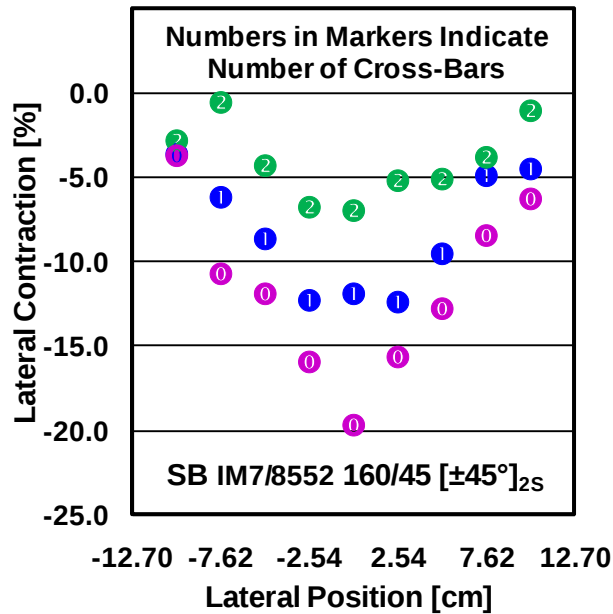
Figure 11: Lateral Contraction of ±45° SB IM7/8552 Panels Stretched by overall 10%
