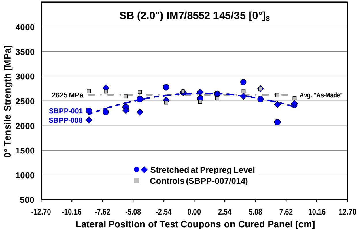
Figure 4: 0° Tensile Strength of SB (2.0'') IM7/8552 Panels “Stretched at Prepreg Level” in Comparison to Control Panels Made from SB Prepreg “As Made”
