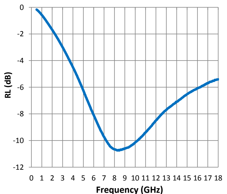
Reflection Loss
