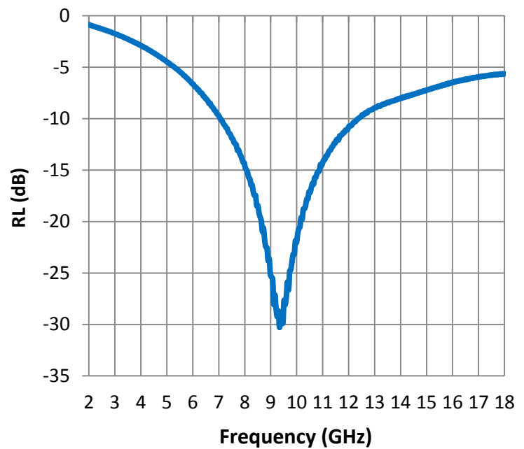
Reflection Loss
