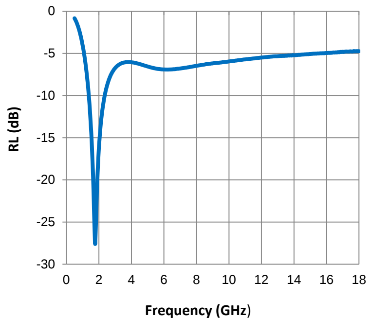
Reflection Loss
