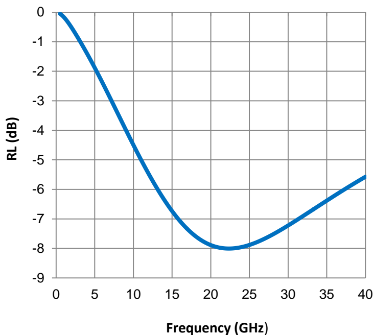
Reflection Loss
