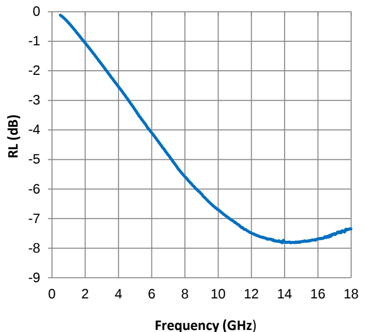
Reflection Loss
