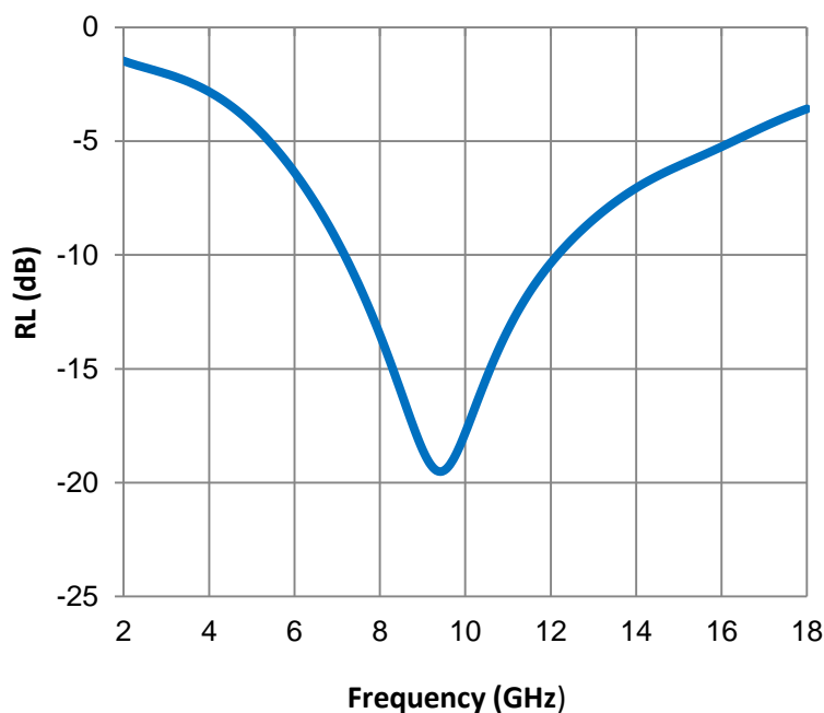
Reflection Loss
