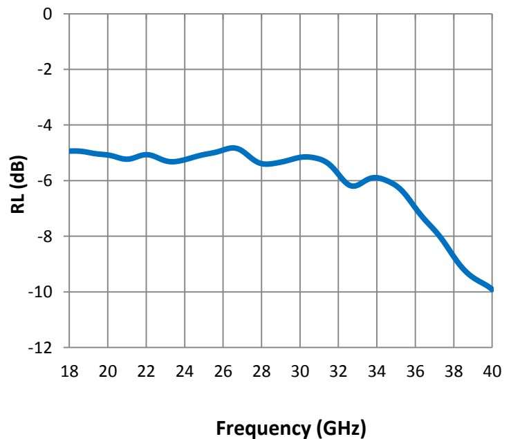
Reflection Loss
