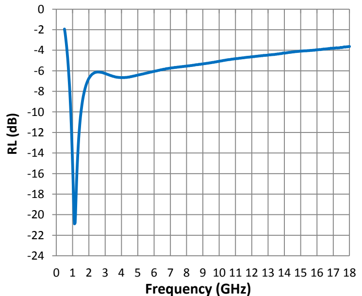
Reflection Loss
