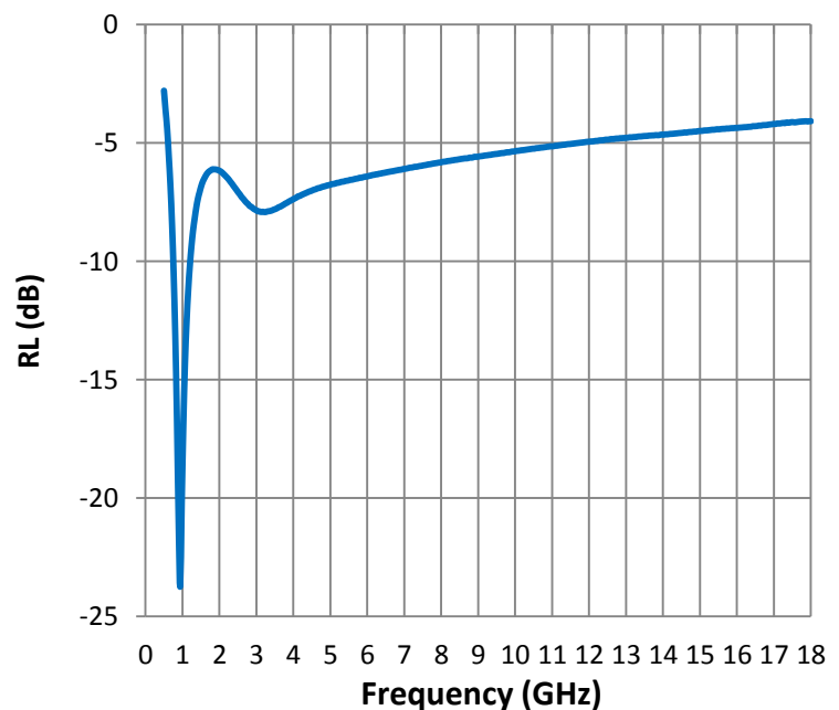
Reflection Loss
