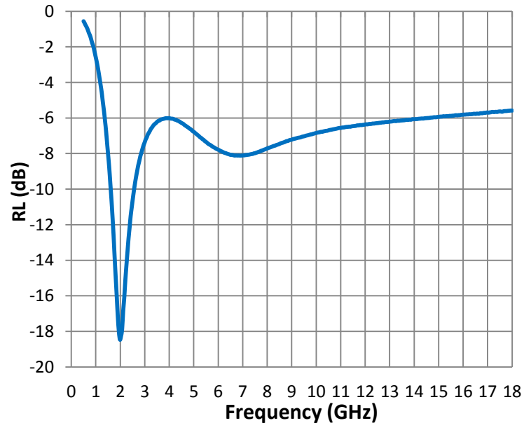
Reflection Loss
