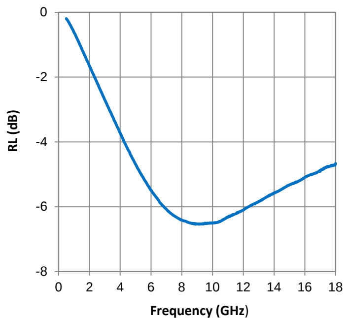
Reflection Loss
