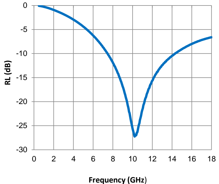
Reflection Loss
