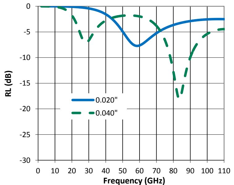
Reflection Loss
