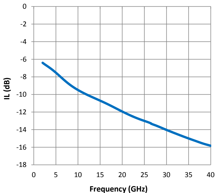
Insertion Loss
