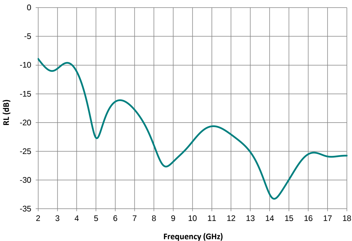
Reflection Loss of RT-10362
