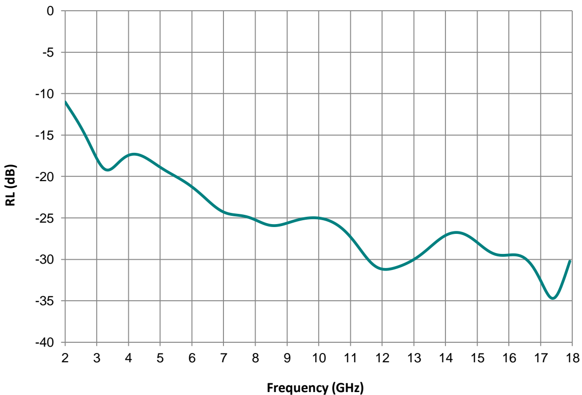
Reflection Loss of RT-10003-3
