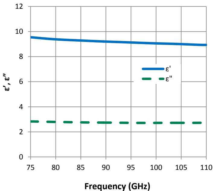
Measured Permittivity
