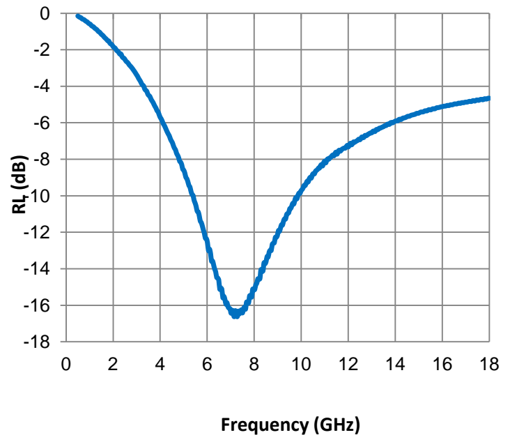
Reflection Loss
