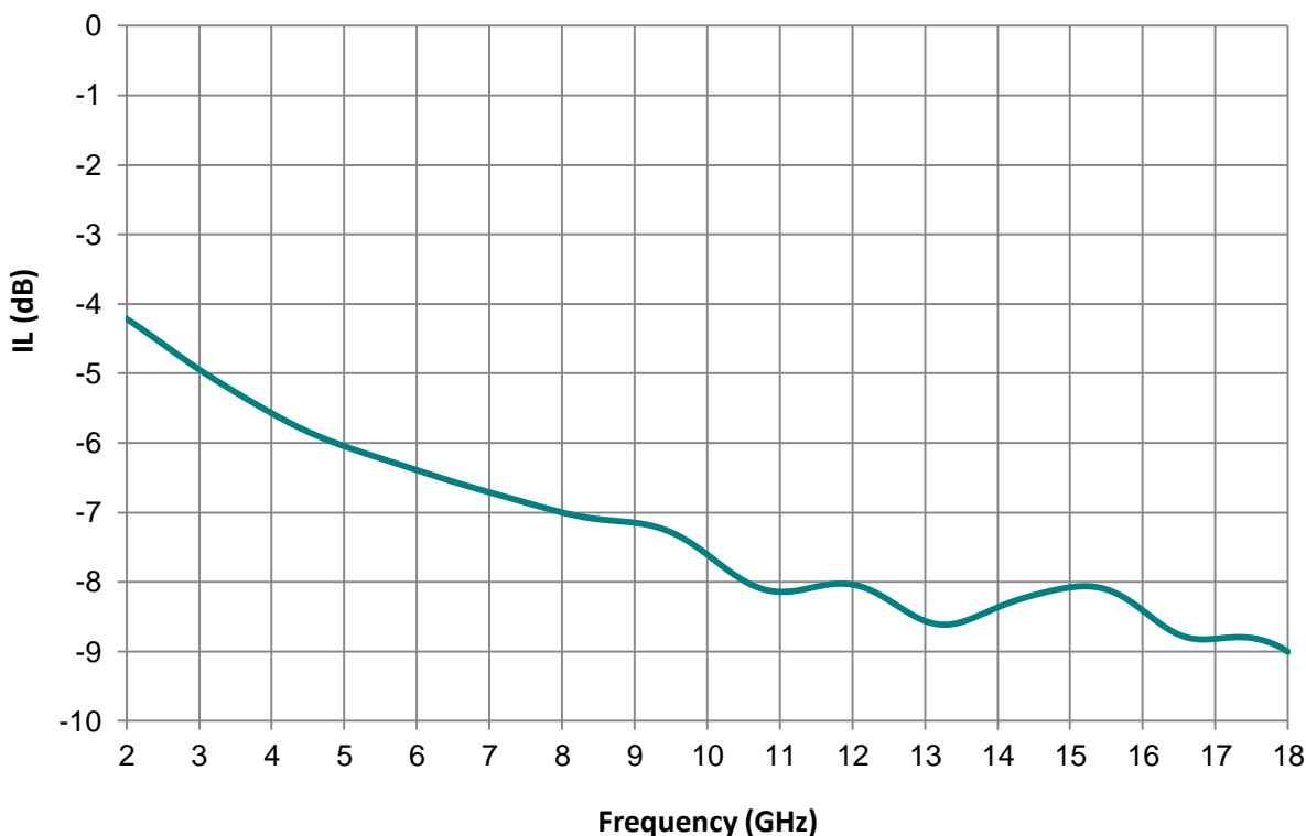
Insertion Loss of LS-12792
