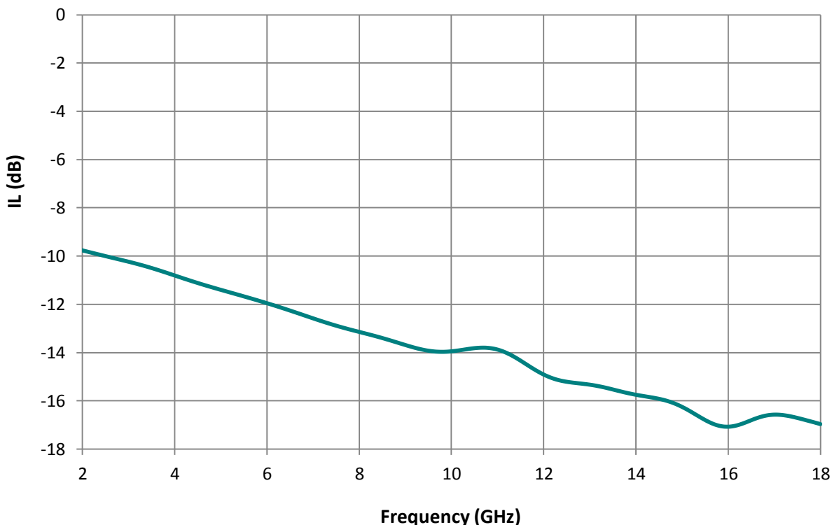
Insertion Loss of LS-11059
