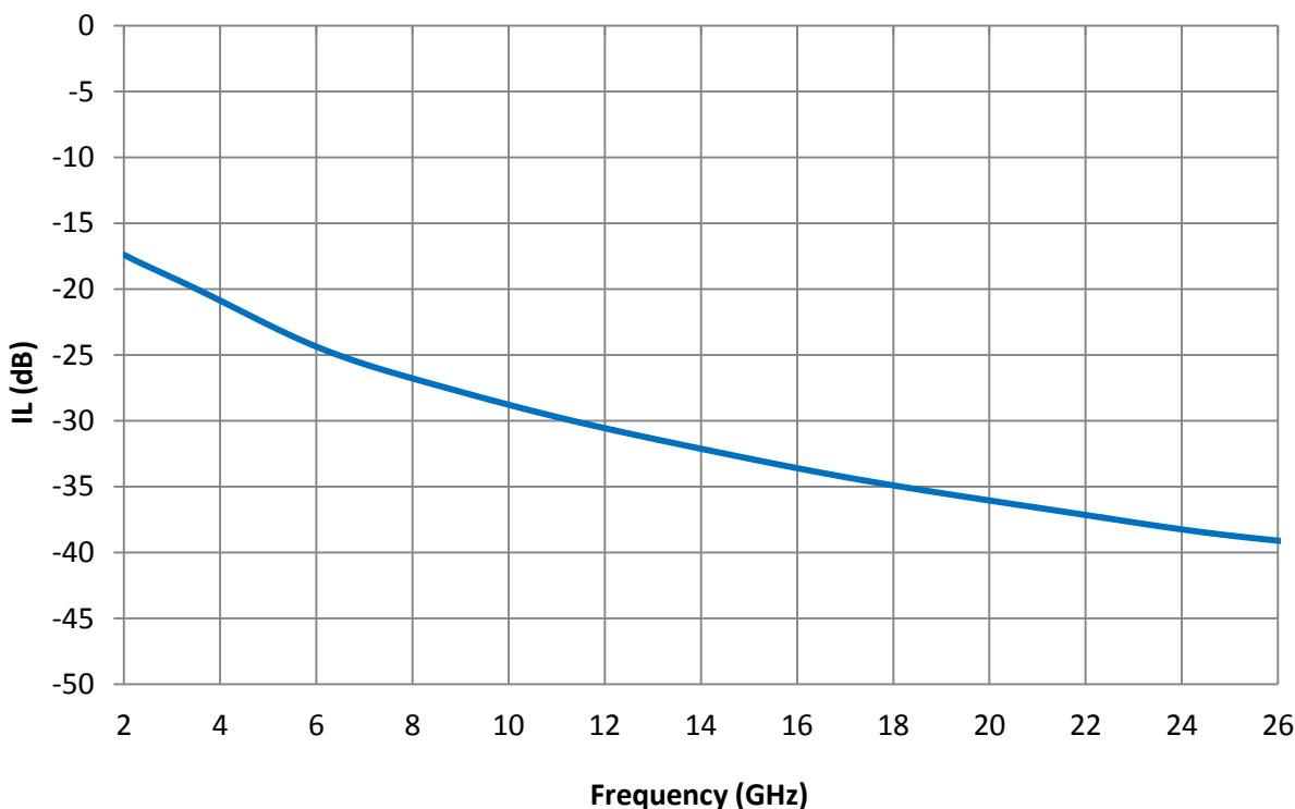
Insertion Loss of LS-10246
