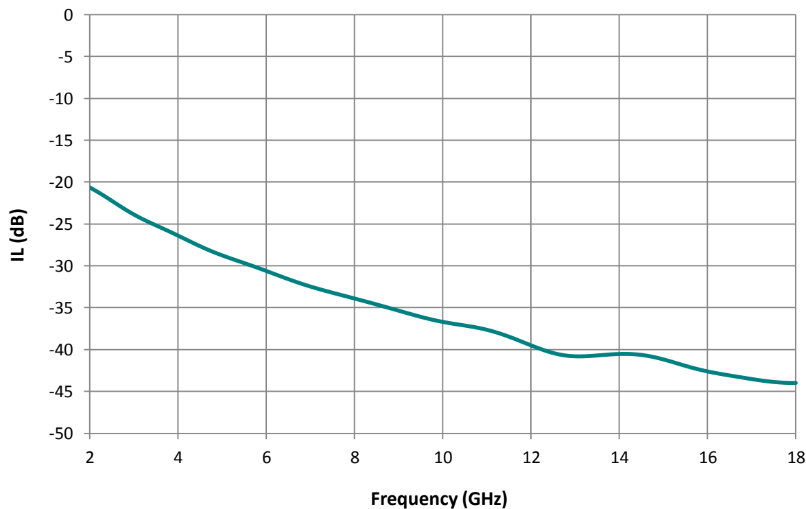
Insertion Loss of LS-10640
