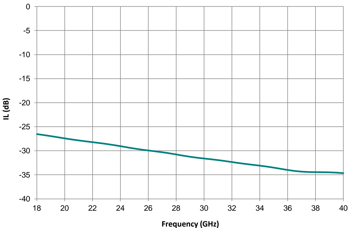
Insertion Loss of LS-10231
