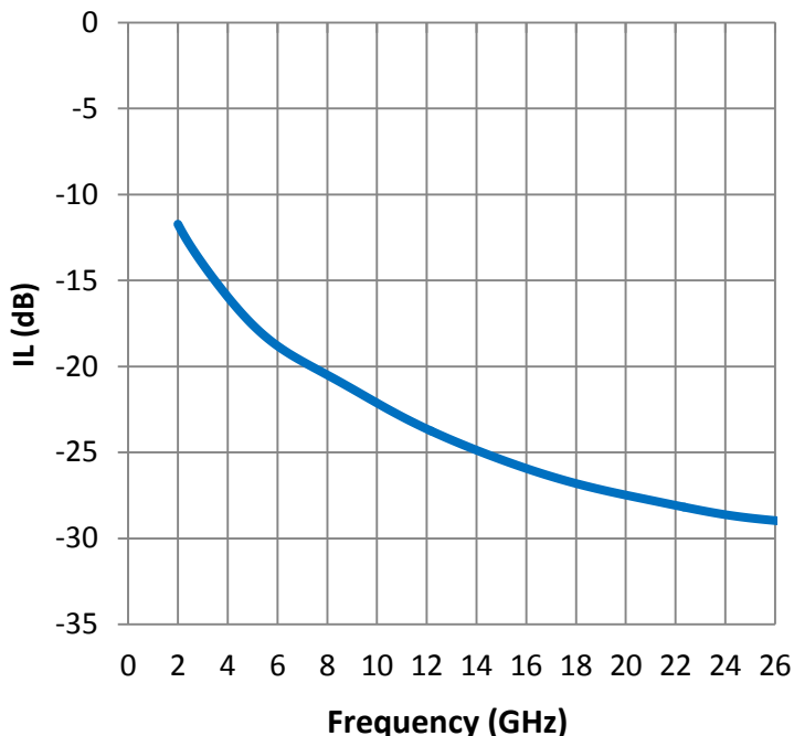
Insertion Loss
