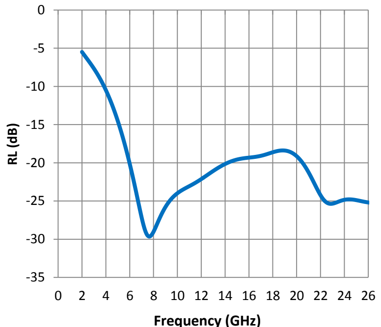
Reflection Loss
