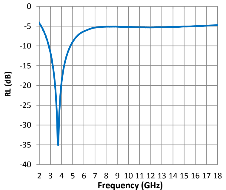
Reflection Loss
