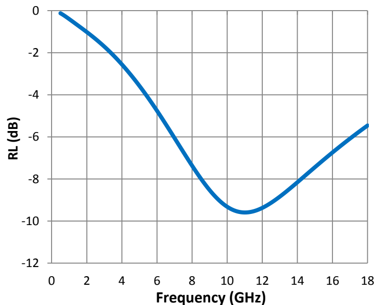
Reflection Loss
