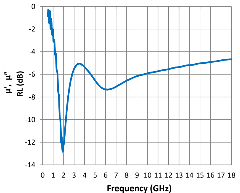
Reflection Loss
