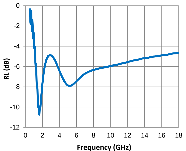
Reflection Loss
