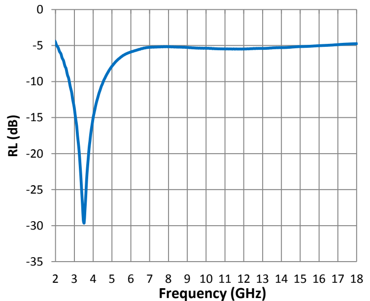
Reflection Loss
