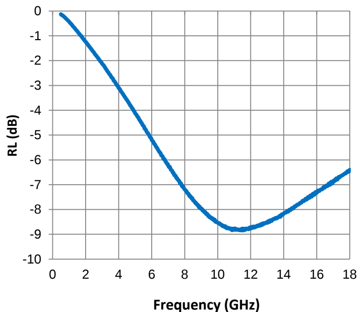
Reflection Loss
