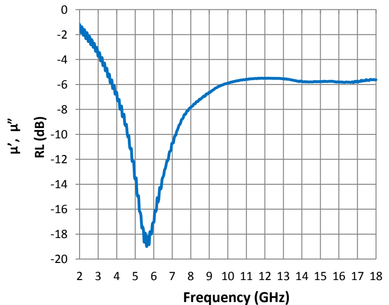
Reflection Loss
