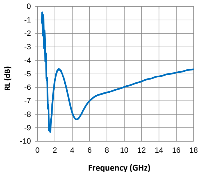
Reflection Loss
