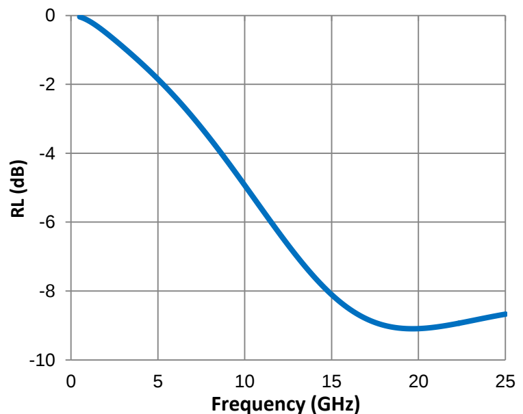
Reflection Loss
