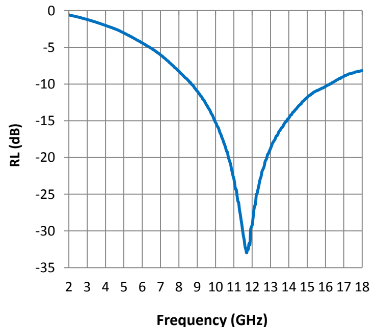
Reflection Loss
