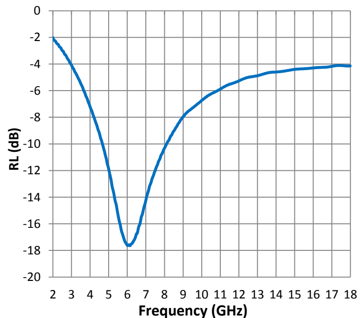
Reflection Loss
