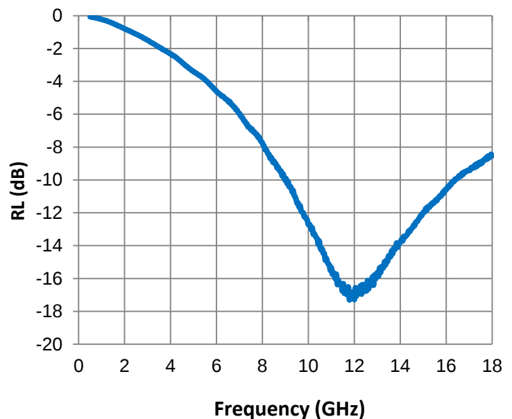
Reflection Loss
