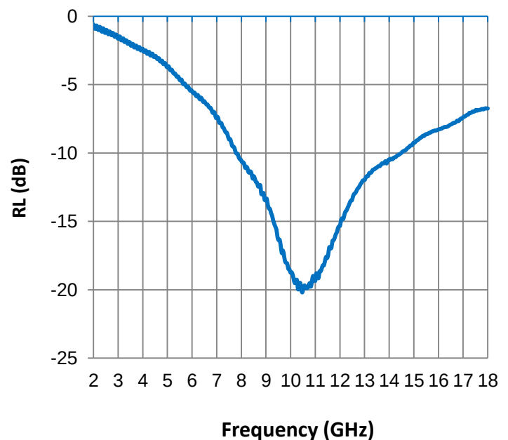
Reflection Loss
