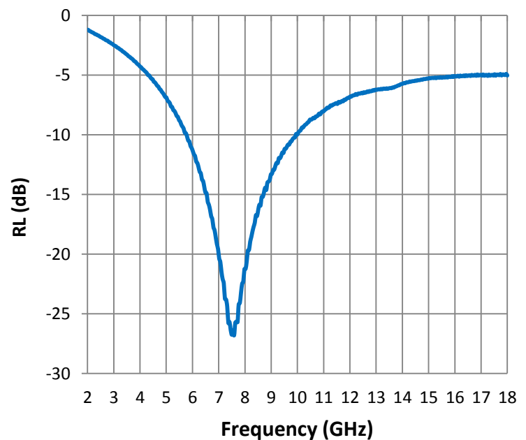
Reflection Loss
