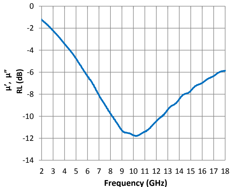
Reflection Loss
