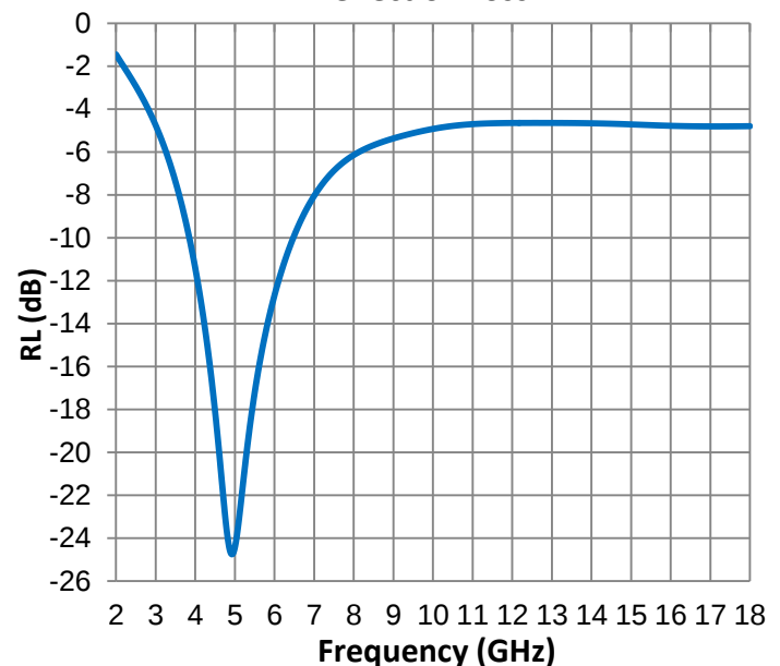
Reflection Loss
