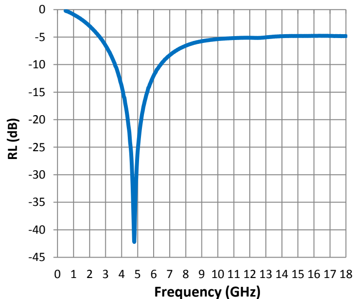
Reflection Loss
