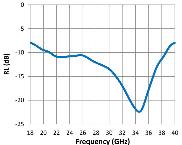
Reflection Loss
