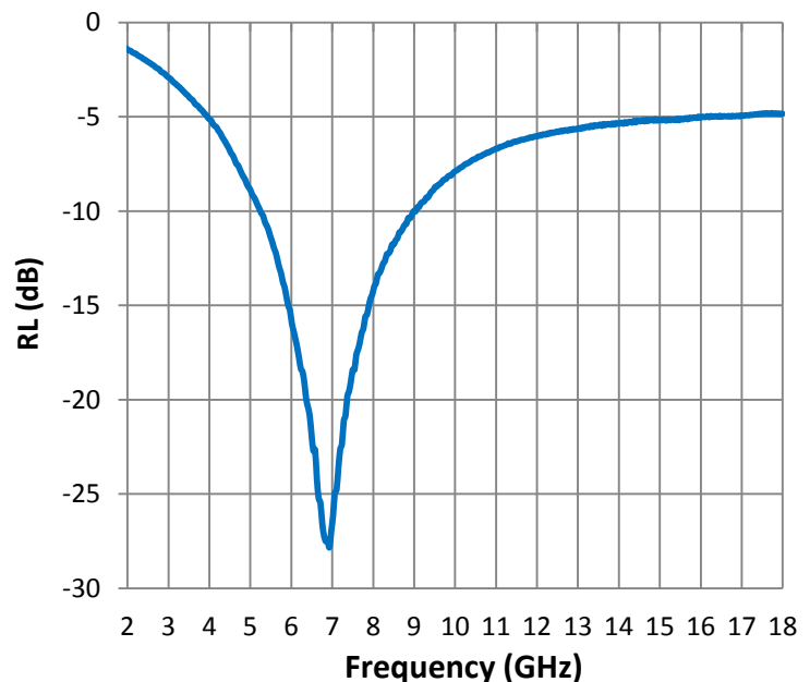
Reflection Loss
