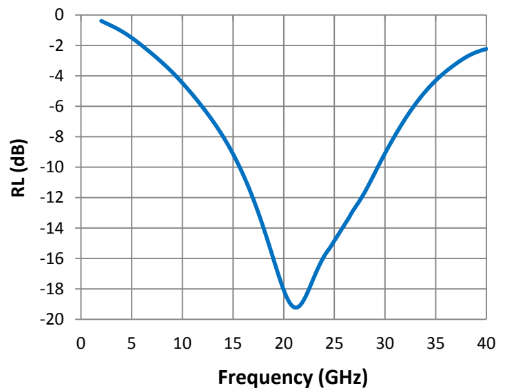
Reflection Loss
