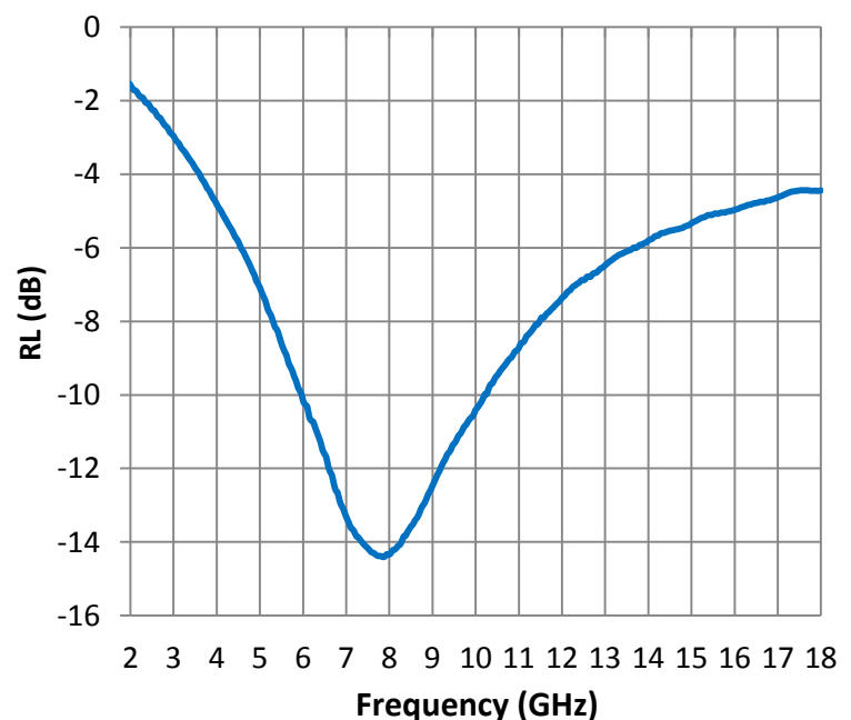
Reflection Loss
